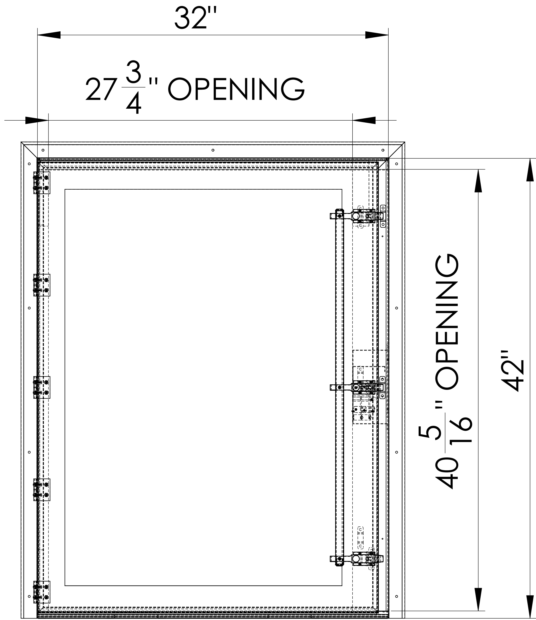
FRONT VIEW
