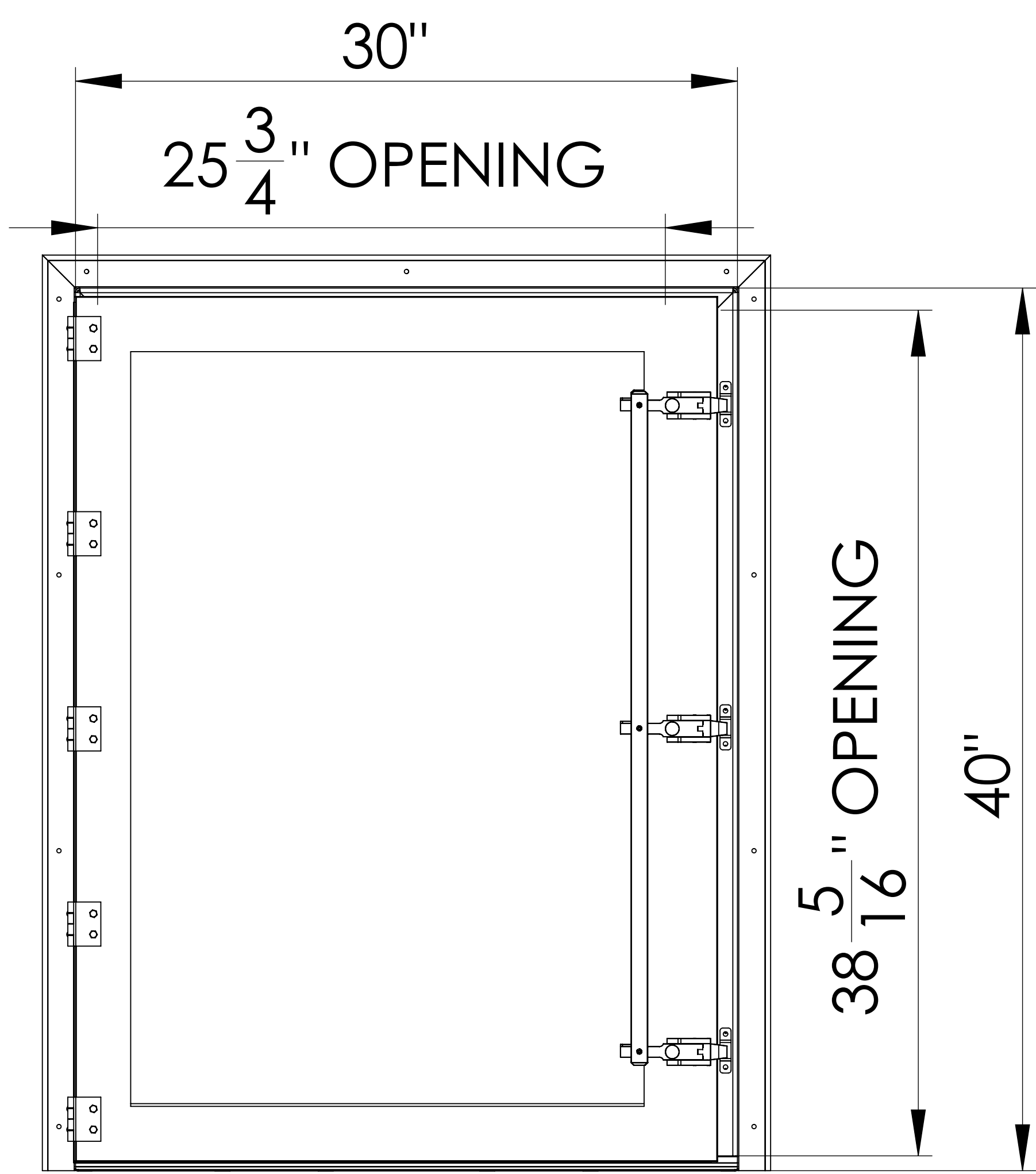
FRONT VIEW
