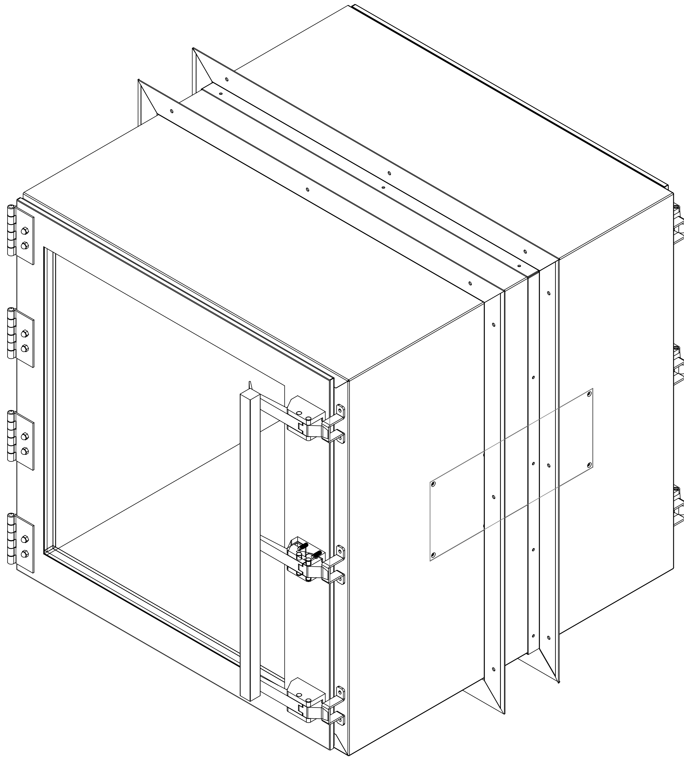
ISOMETRIC VIEW
