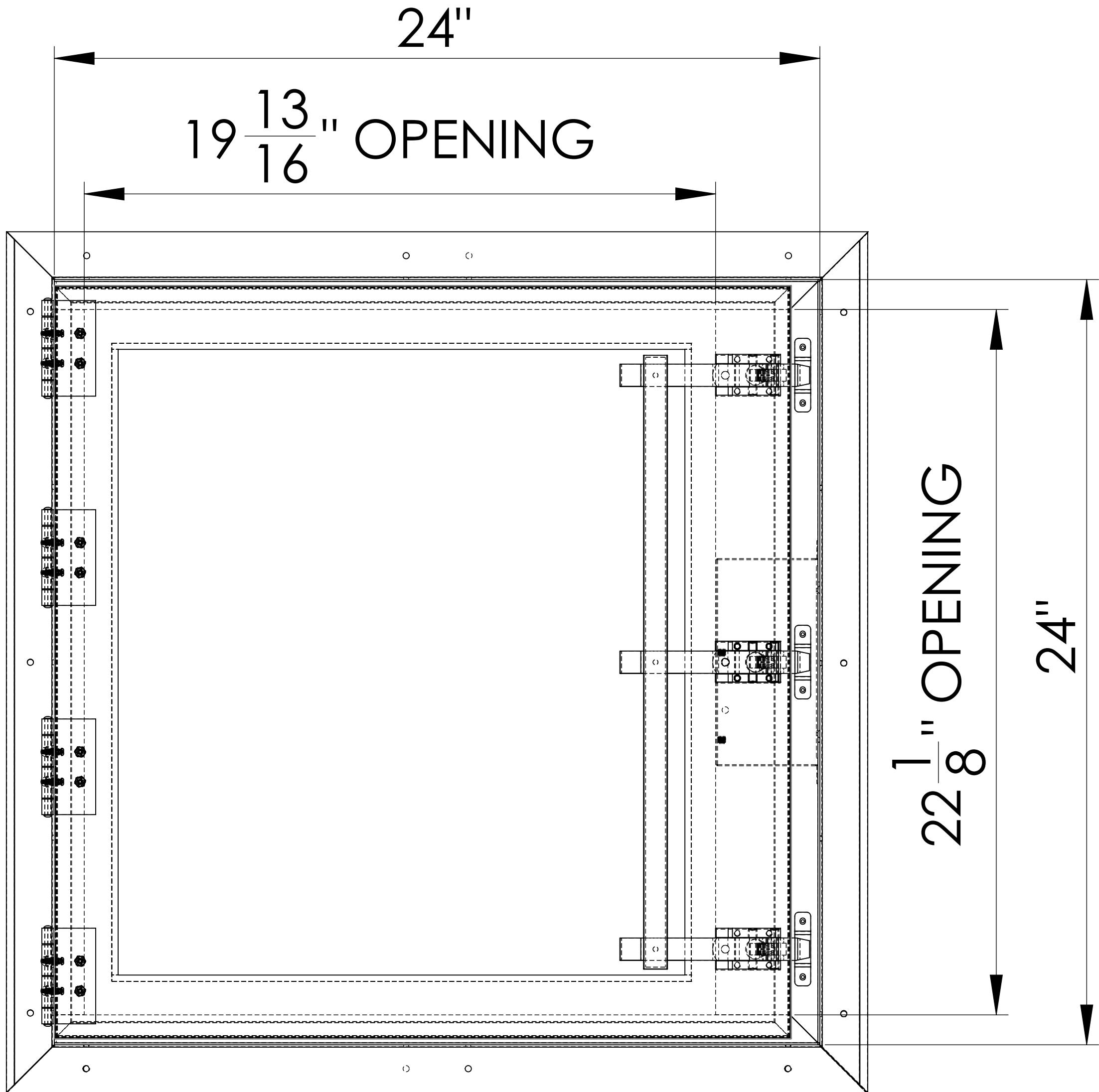
FRONT VIEW
