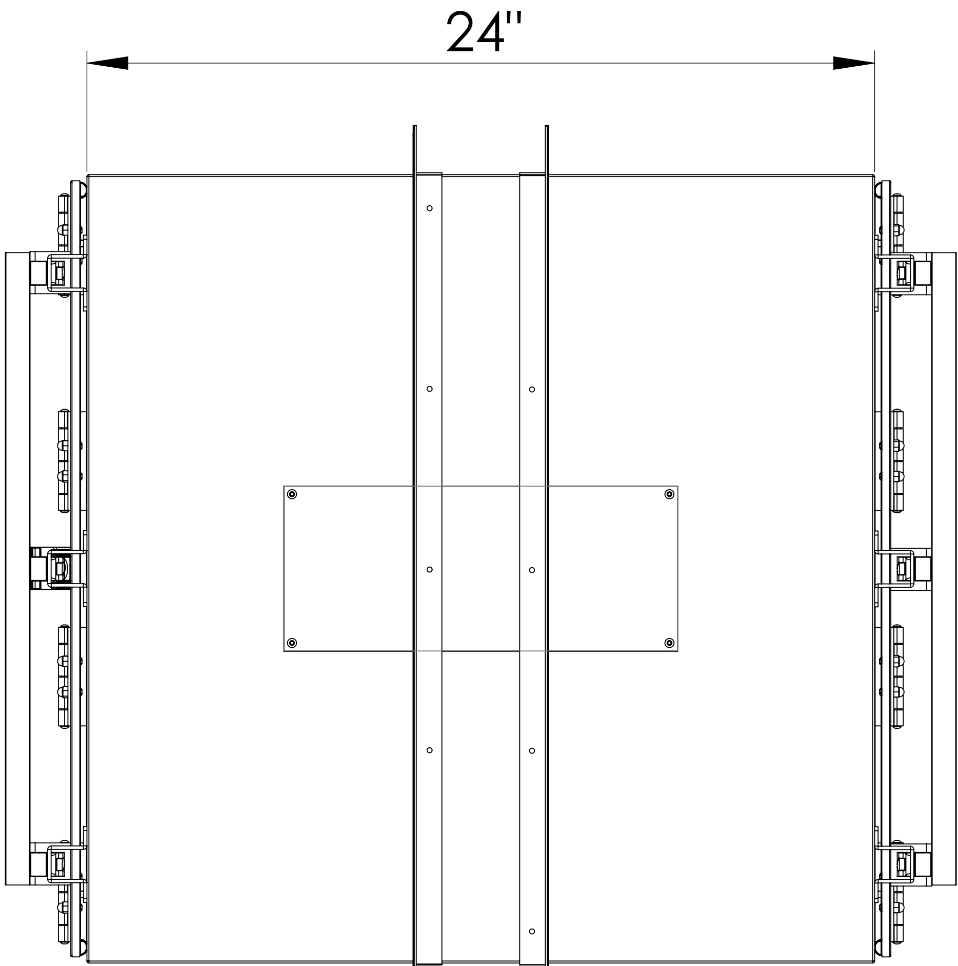
SIDE VIEW
