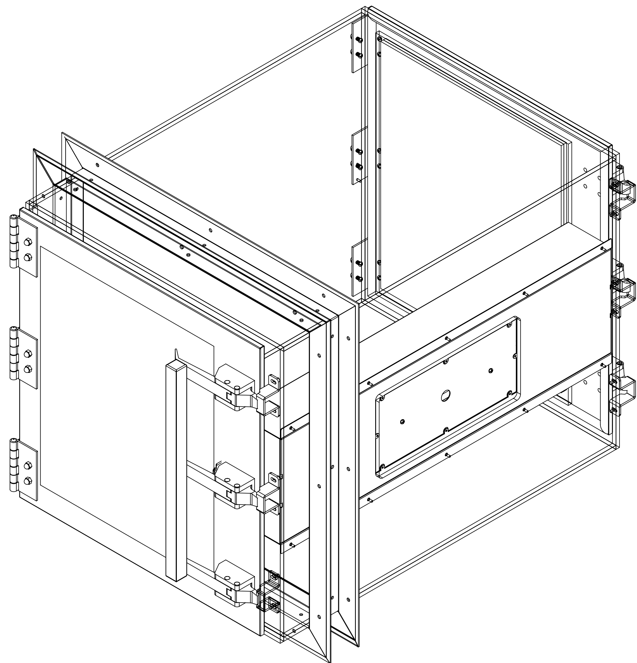
ISOMETRIC VIEW
