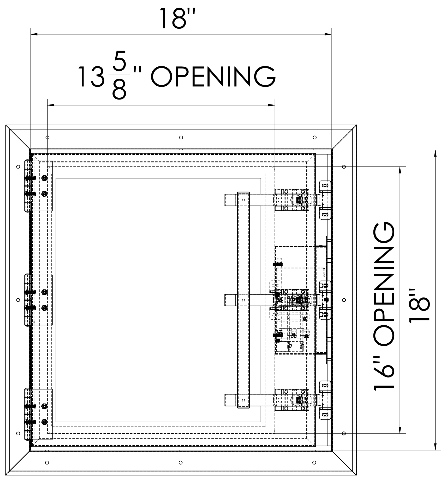
FRONT VIEW
