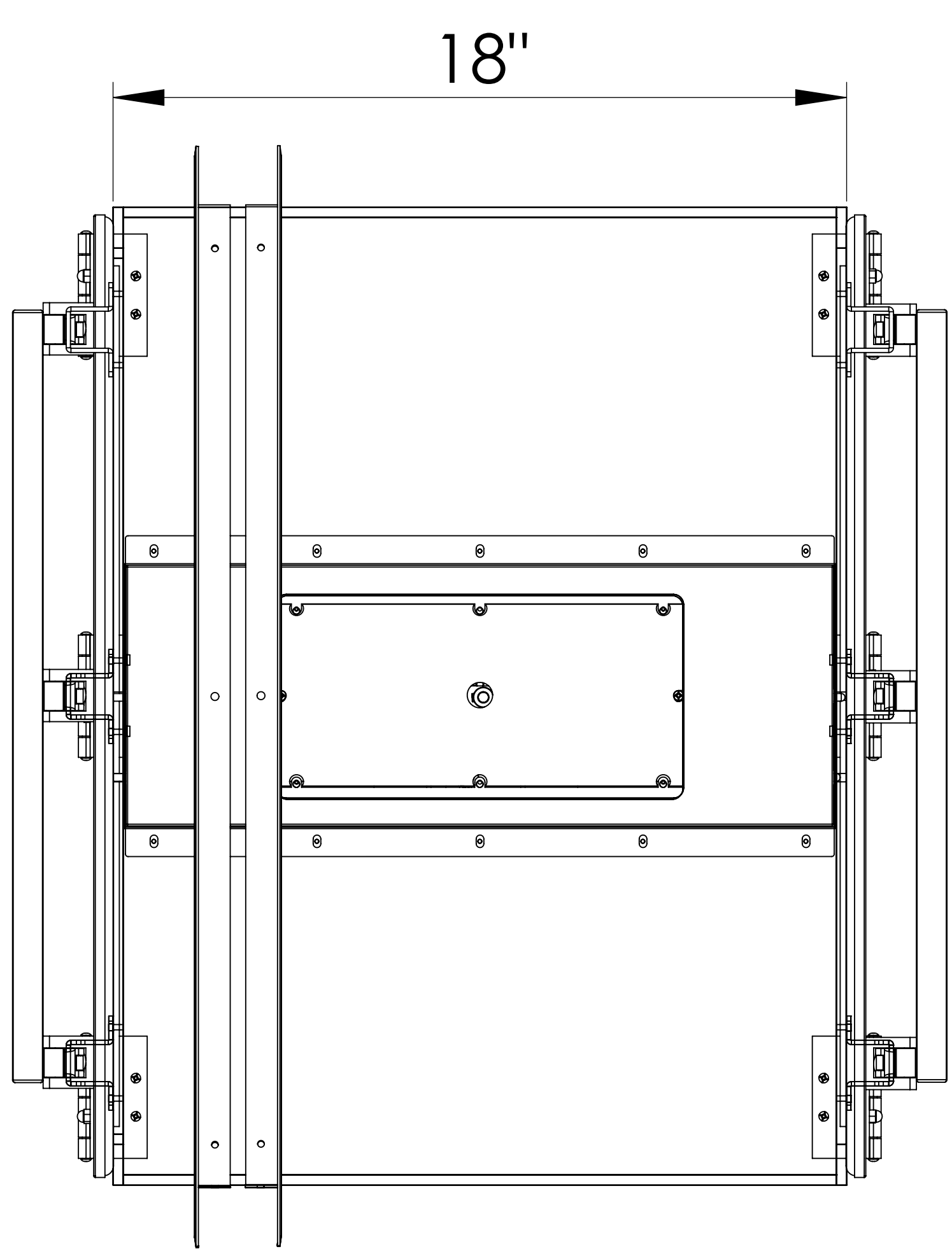
SIDE VIEW
