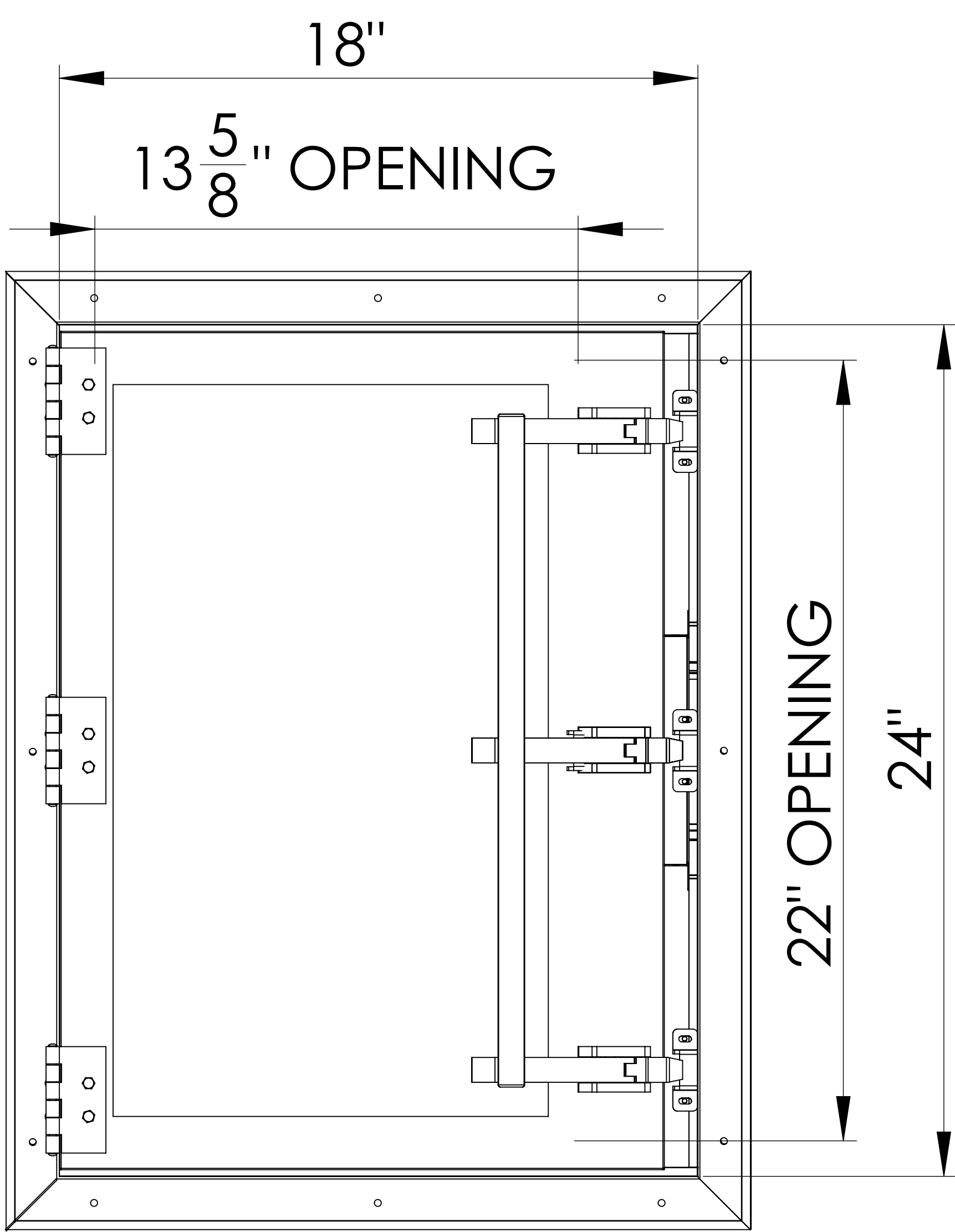
FRONT VIEW
