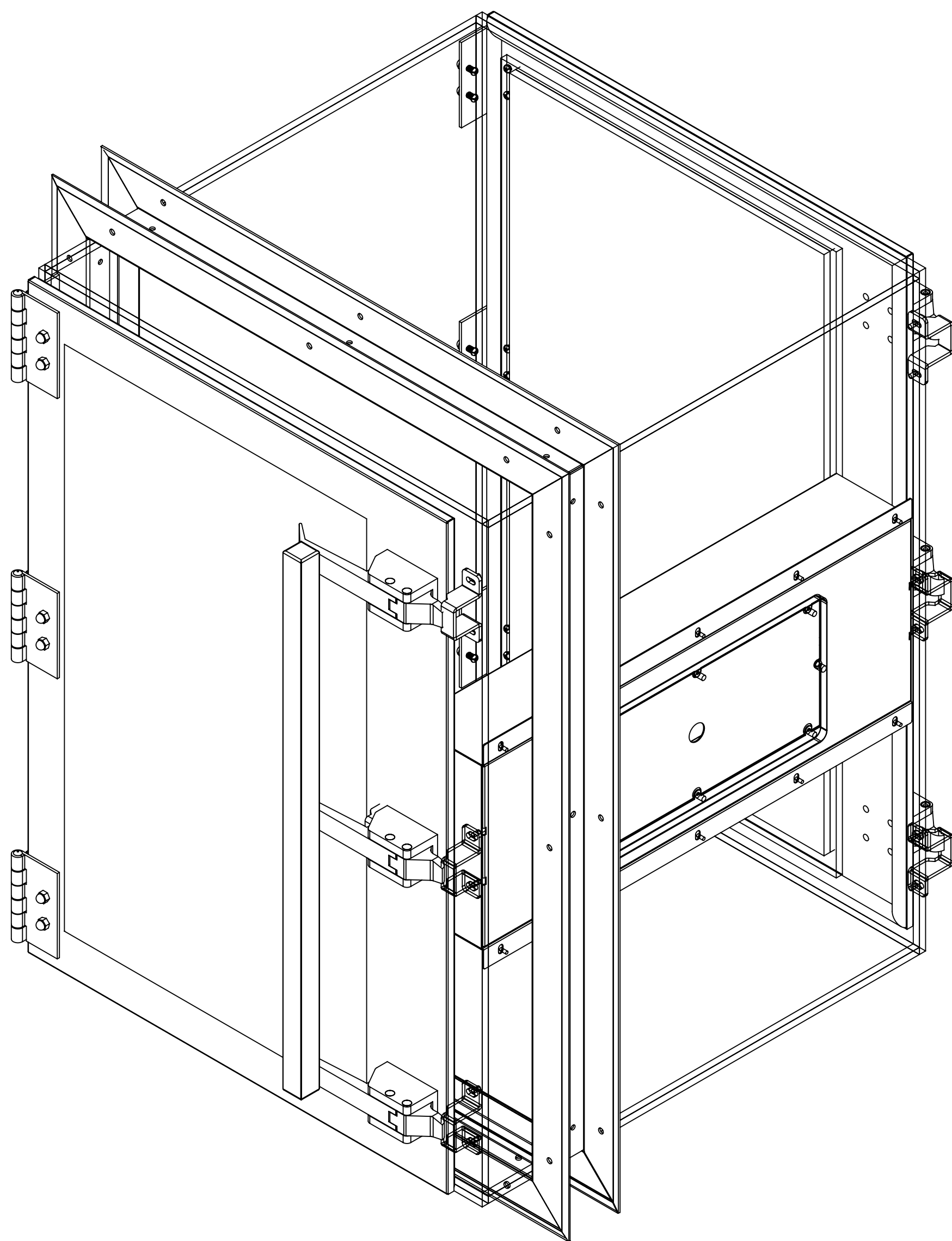
ISOMETRIC VIEW
