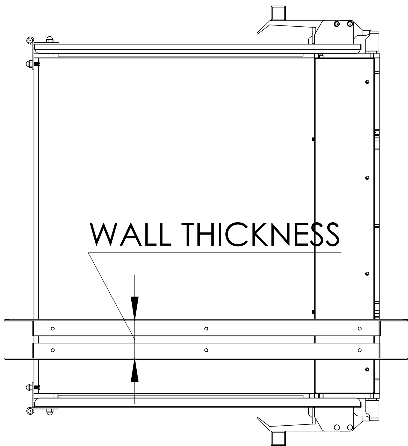
TOP VIEW
