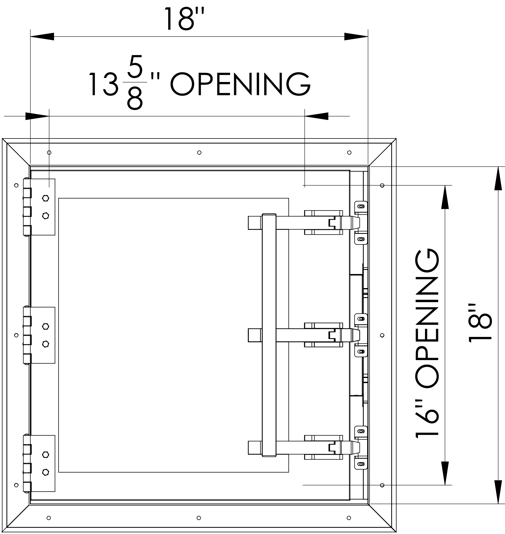
FRONT VIEW
