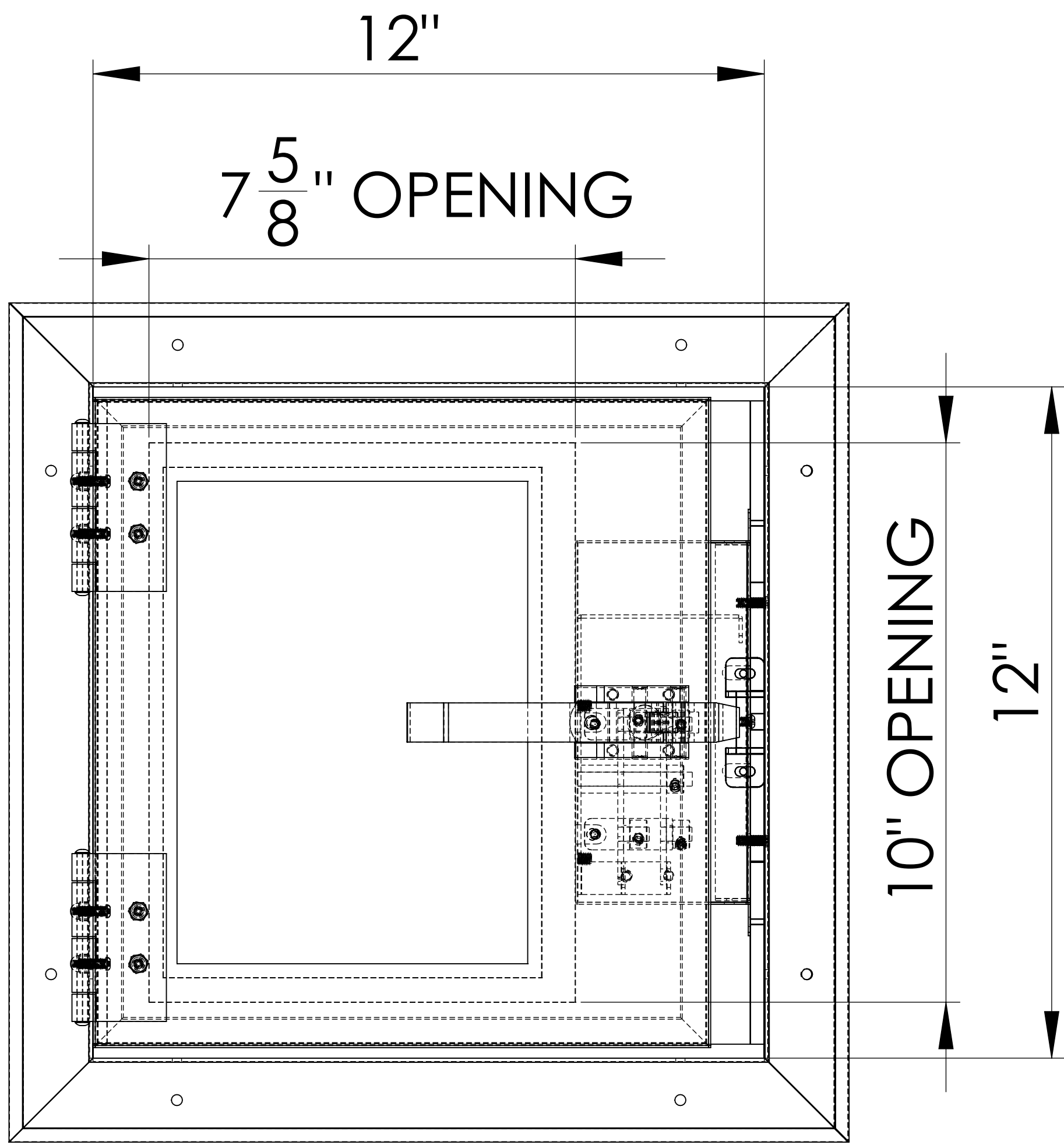
FRONT VIEW
