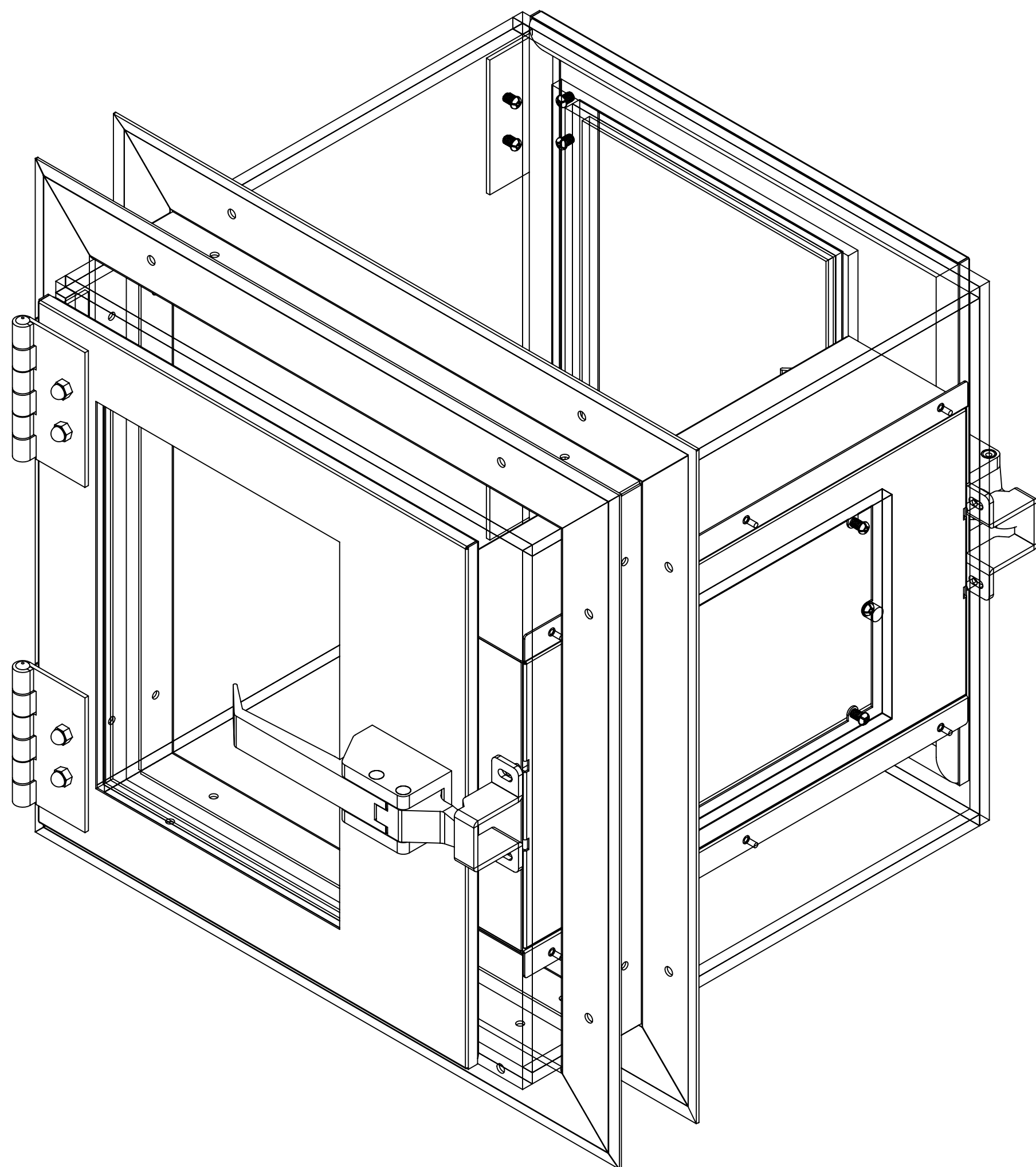
ISOMETRIC VIEW
