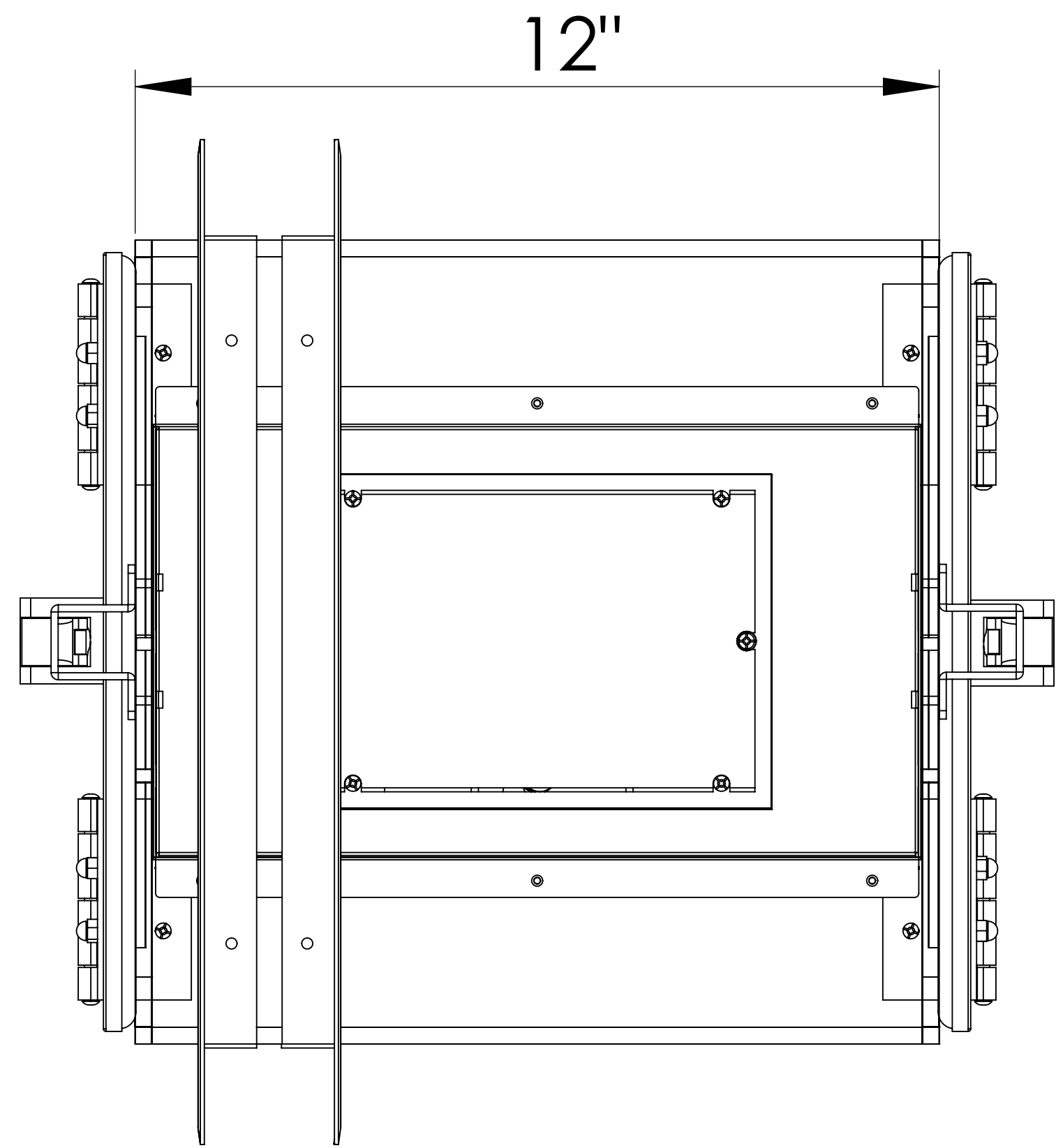
SIDE VIEW
