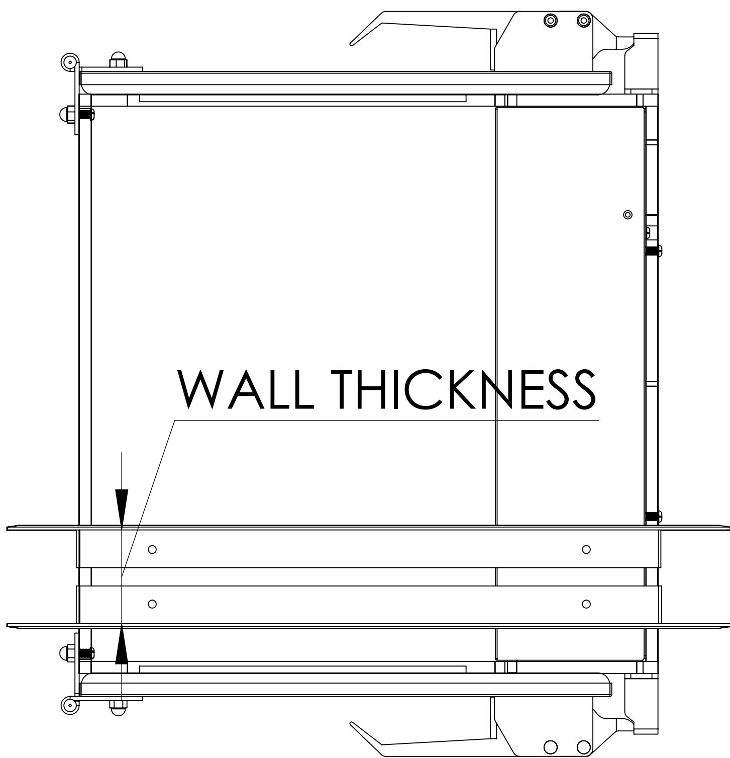
TOP VIEW
