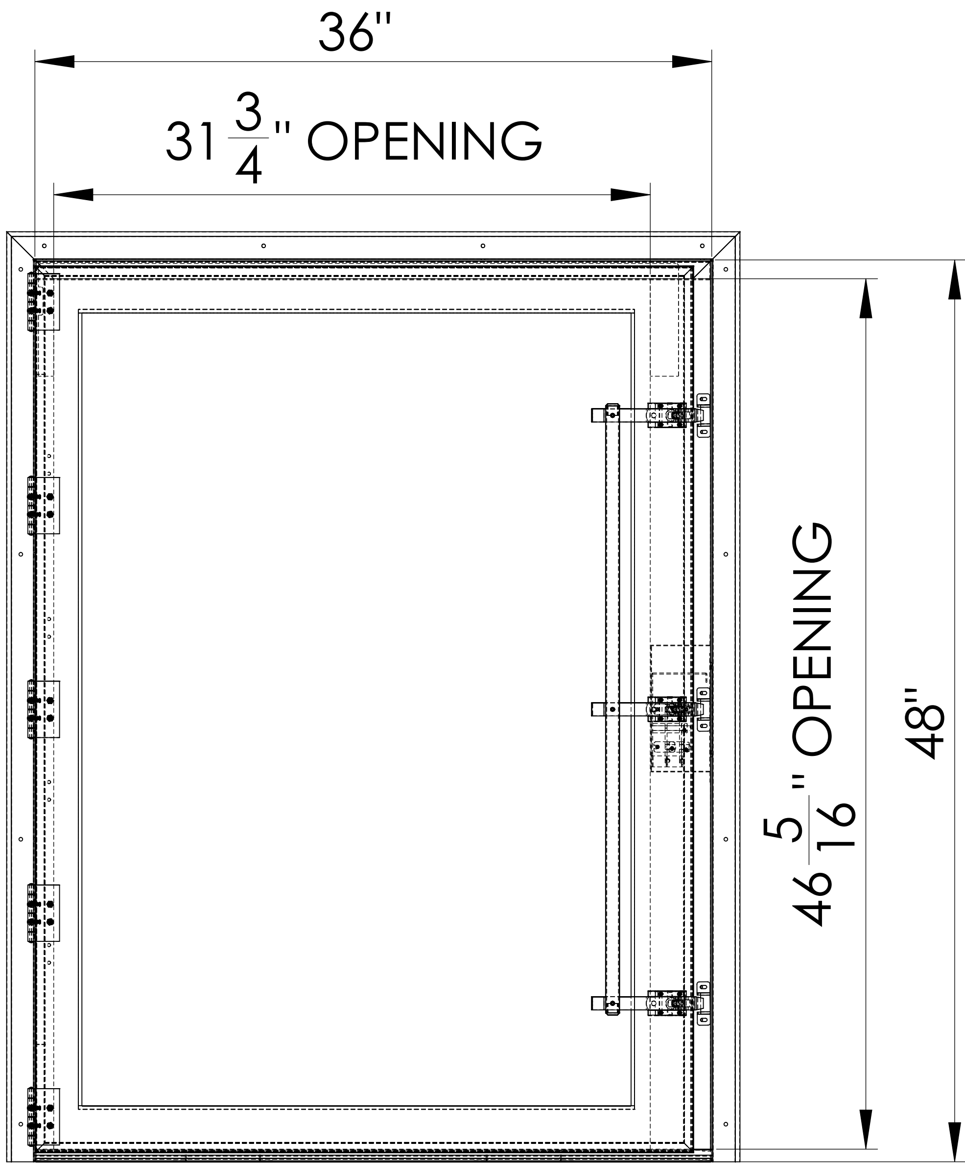
FRONT VIEW
