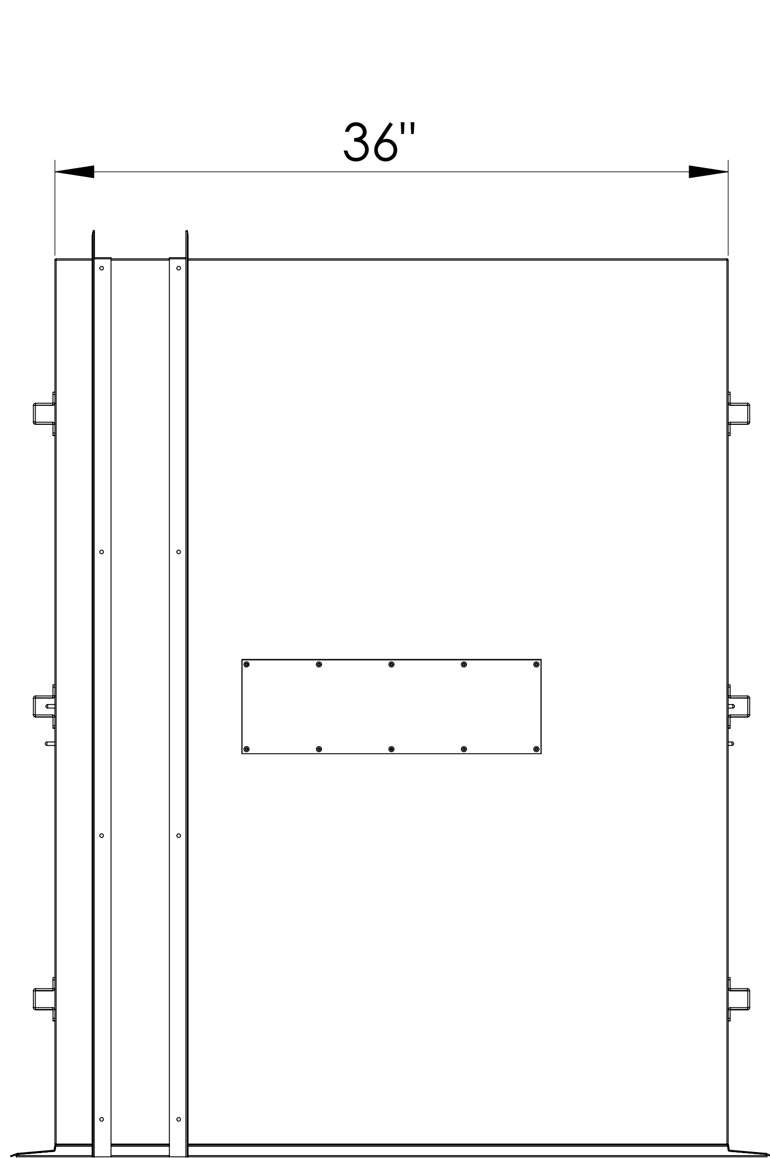
SIDE VIEW
