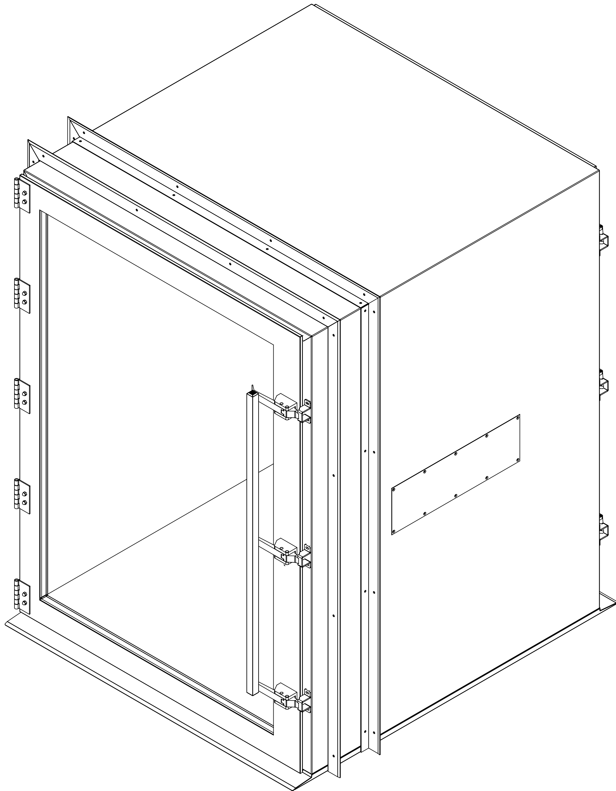
ISOMETRIC VIEW
